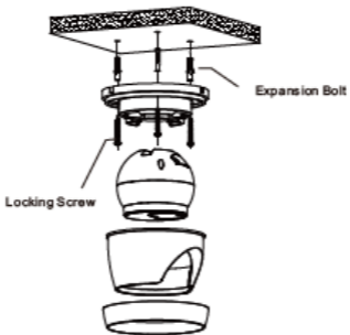
Figure 2-3 fix the camera onto wall/ceiling
