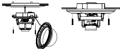
Figure 2-6 Fix the Camera to the Mount
