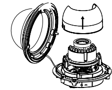
Figure 2-2 Remove the Bubble
