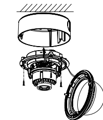
Figure 2-3 Fix the Camera to the Ceiling
